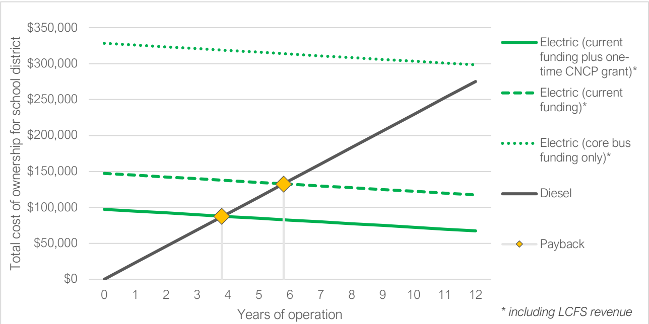
Figure 11. Up-front costs, operating costs, and LCFS revenues for school district over the 12-year bus lifetime for Type D buses
