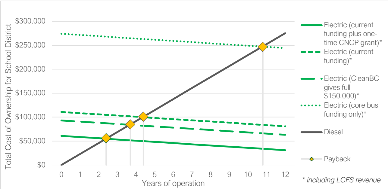
Figure 10. Up-front costs, operating costs, and LCFS revenues for school district over the 12-year bus lifetime for Type C buses
