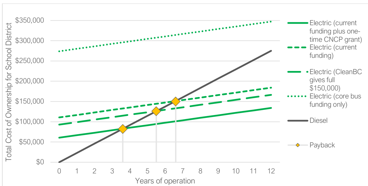
Figure 8. Up-front and operating costs to school district over the 12-year bus lifetime for Type C buses, under different funding scenarios
