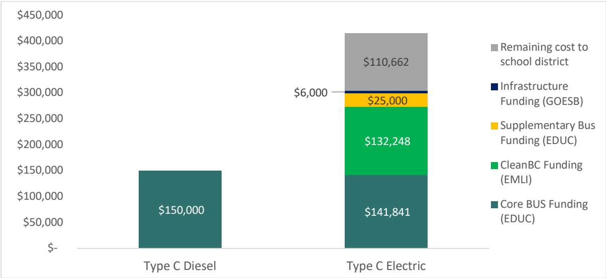
Figure 1. Breakdown of funding sources for Type C school buses
