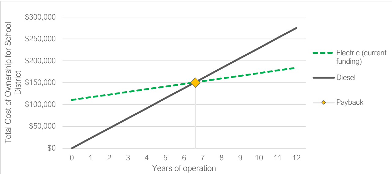
Figure 2. Up-front and operating costs to school district over the 12-year bus lifetime for Type C buses
